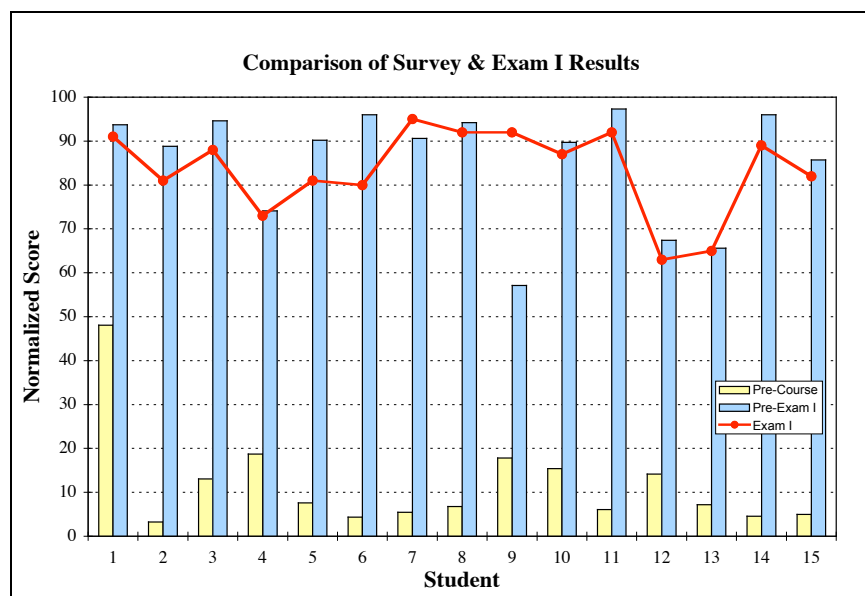
Figure 1. Histogram plot of pre-course and pre-exam knowledge survey and first mid-term exam results for students ( n = 15 ) in the Macalester College Dynamic Earth and Global Change course. Survey results are normalized to 100 for comparison with exam results. For most students, the pre-exam survey results correlate well ( r = 0.90 for all students excluding #9) with exam score. Students 12 and 13 indicated a lack of preparation on the pre-exam I survey, and their exam scores reflect lower levels of understanding. Student 9 indicated low confidence on the pre-exam I survey, but completed a very strong exam suggesting lack of self confidence, poor self-assessment skills, or additional pre-exam preparation after taking the survey.
