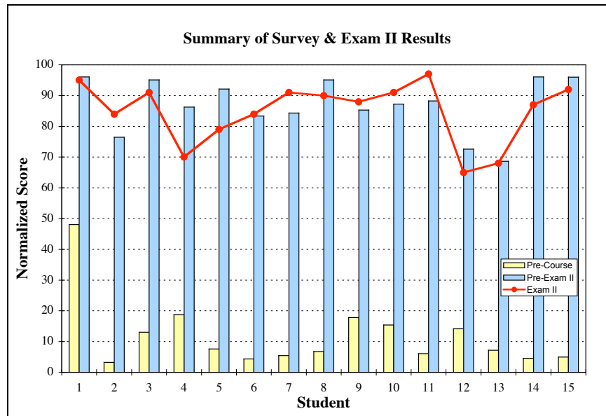
Figure 2. Histogram plot of pre-course and pre-exam knowledge survey and second midterm exam results for students ( n = 15 ) in the Macalester College Dynamic Earth and Global Change course. For most students, pre-exam II knowledge survey results correlate well ( r = 0.70 ) with exam score. As in the first exam, students 12 and 13 indicated a lack of confidence on the knowledge survey and their exam scores reflect lower levels of understanding. Note that student 9 had a more realistic assessment of content mastery in the pre-exam survey before the second exam (compare with Figure 1).
